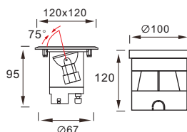
IG0120AST/JSQ beam angle adjustable
