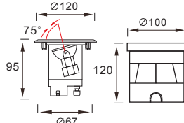
IG0120AST/JR beam angle adjustable
